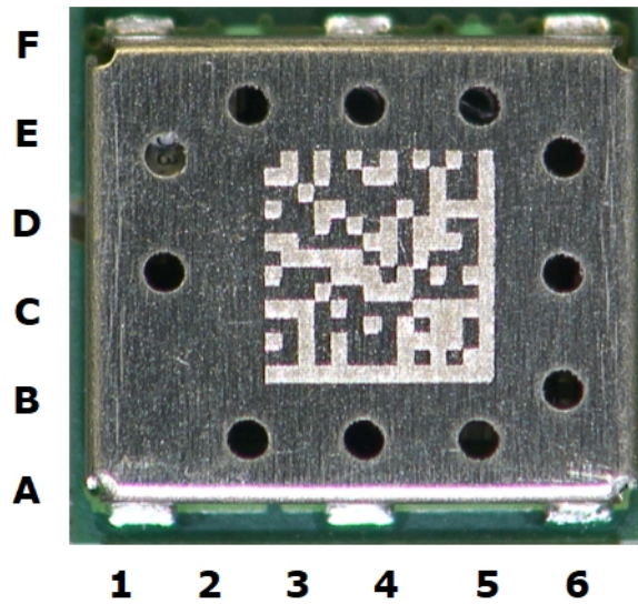
Topview of GNS7000 from current production. *note1
